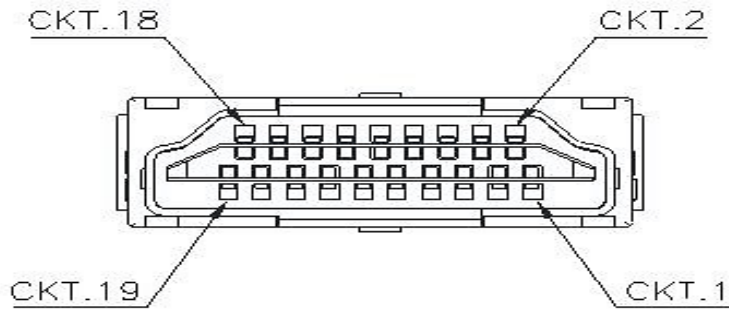
HDMI Type A Connector Pin Assignment
